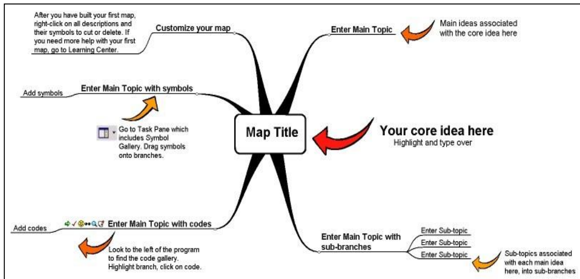
Figure 8 – MindManager Example
